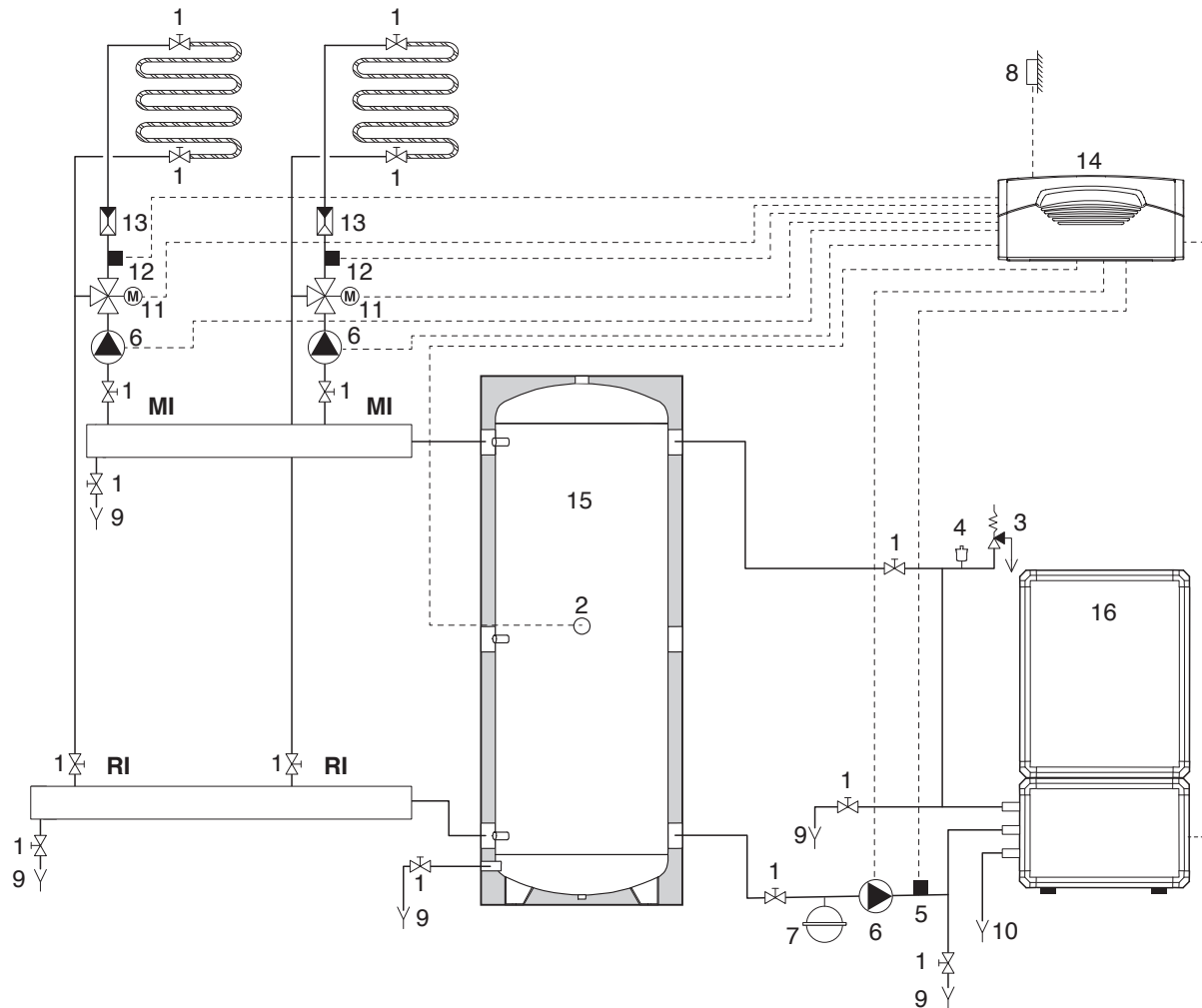
TYPICAL WATER SYSTEM SCHEMATIC
