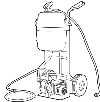
Heat transfer fluid filling pump (accessory). A manual bleed valve is not required if this pump is used.
