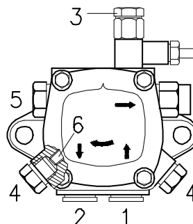
RL 100 - RL 130 PUMPE SUNTEC AJ6 CC
