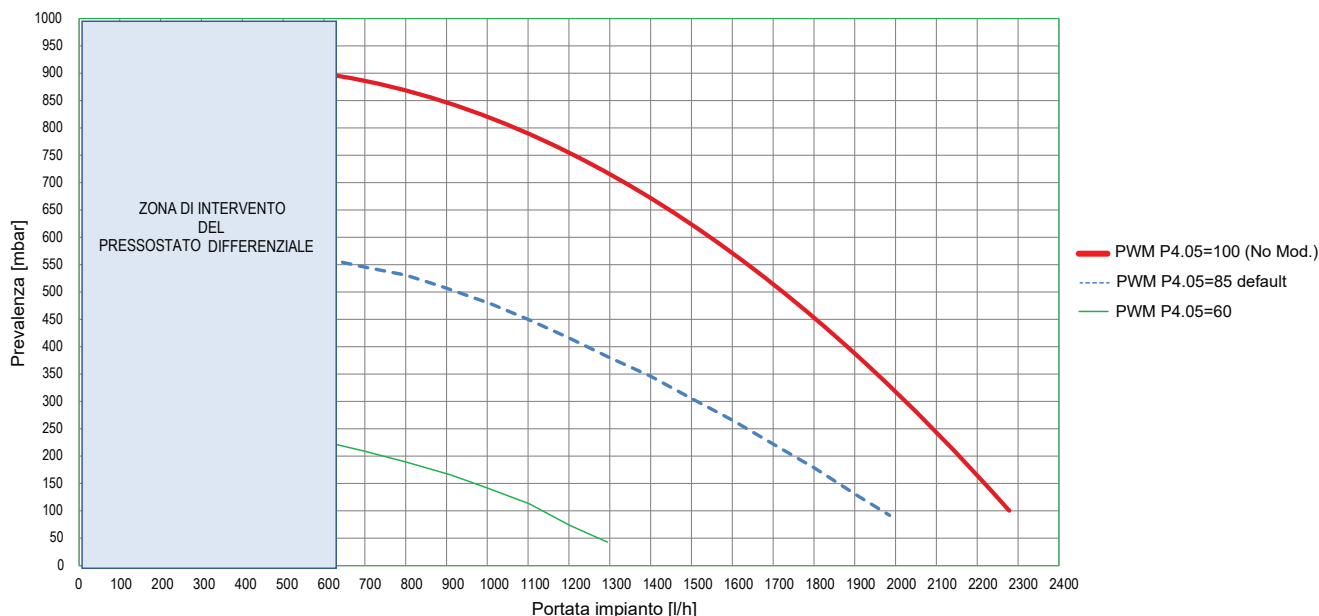
CONDEXA 55-70 HPR
