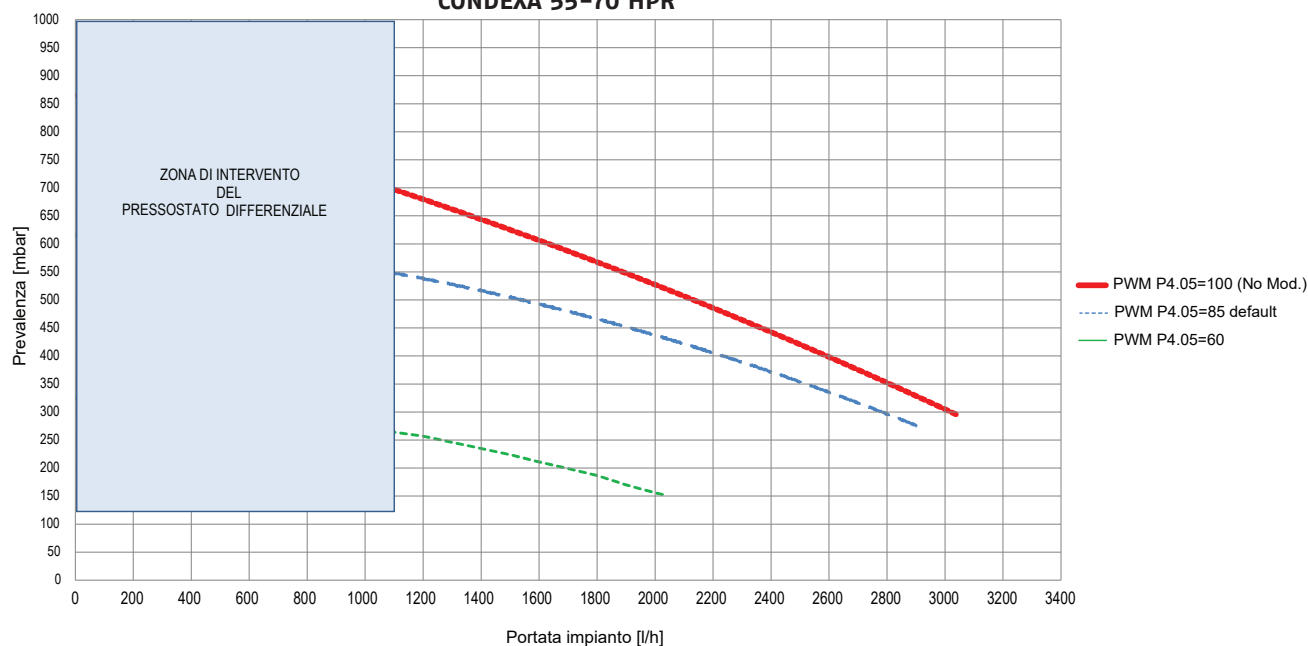
CONDEXA 55-70 HPR
