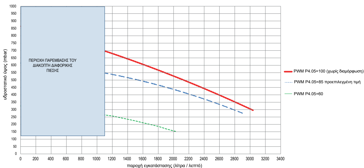
CONDEXA HPR 55-70
