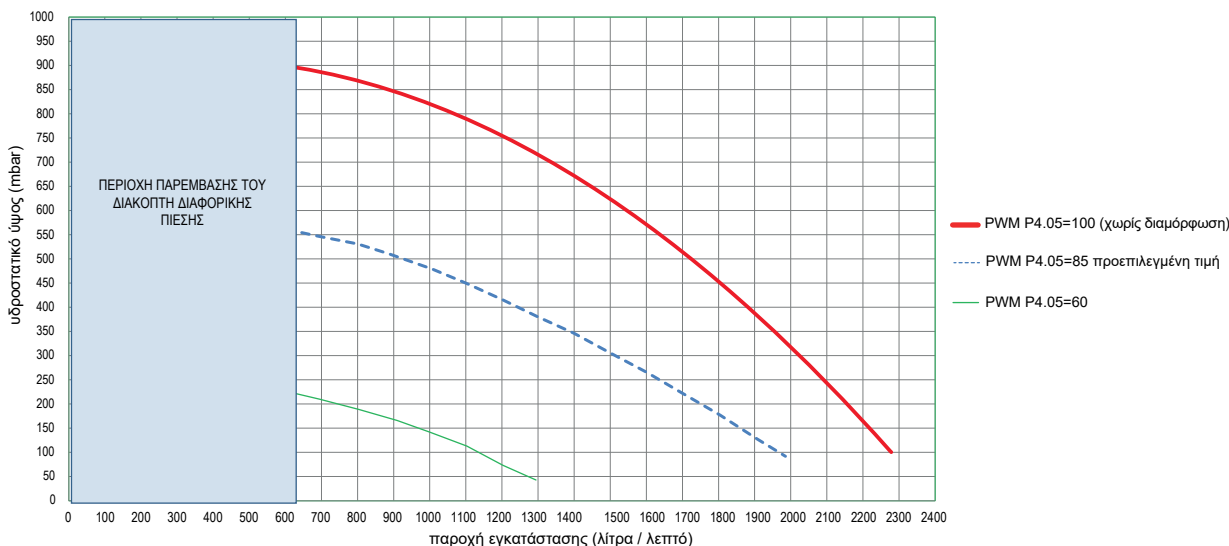
CONDEXA HPR 35-45
