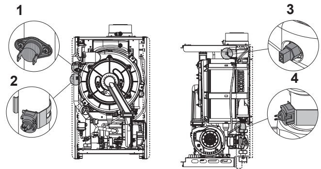
CONDEXA HPR 55-70
