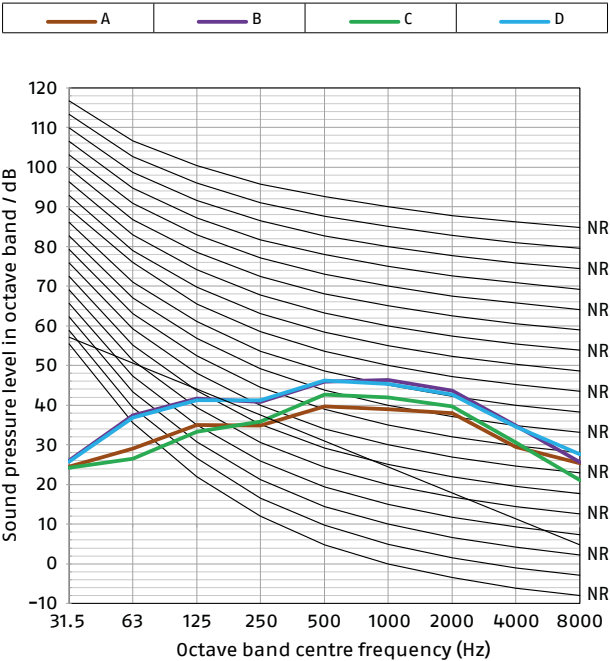
Cooling A35W18
