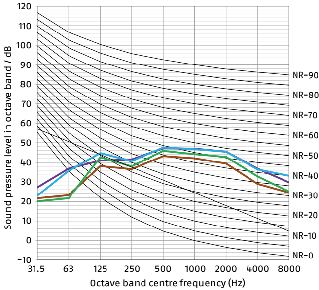
Cooling A35W7
