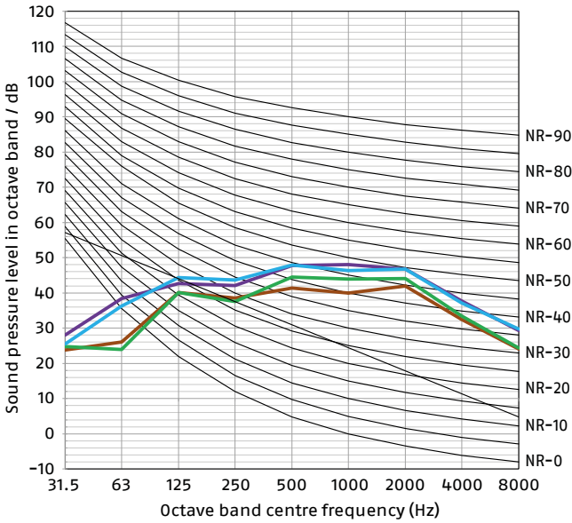
Cooling A35W18
