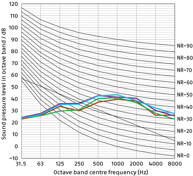
Cooling A35W7
