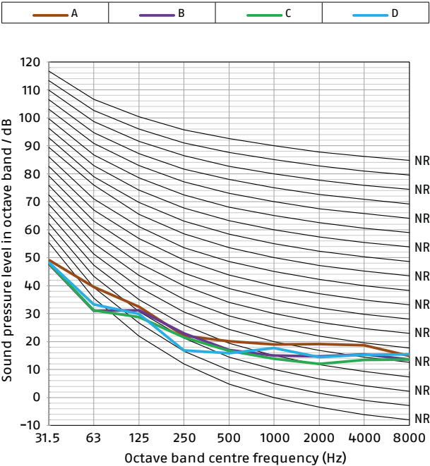
Cooling A35W18
