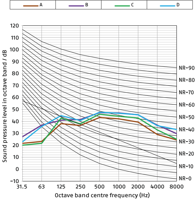
Heating A7W45
