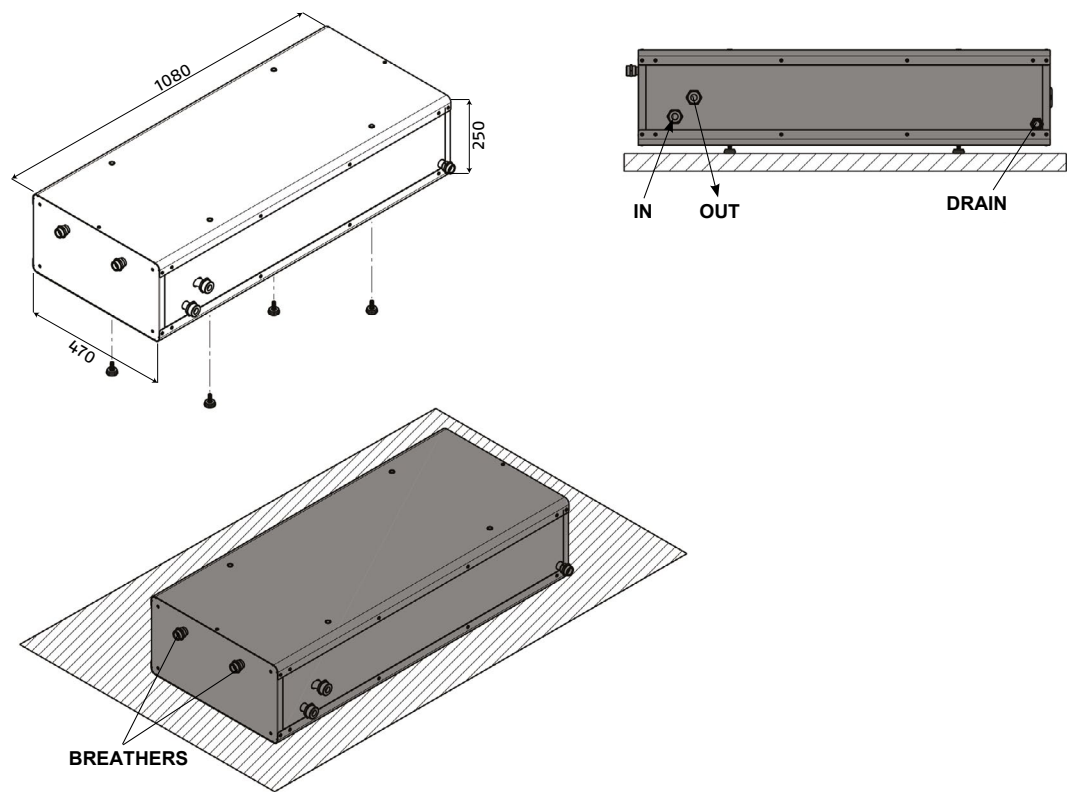
FLOOR INSTALLATION
