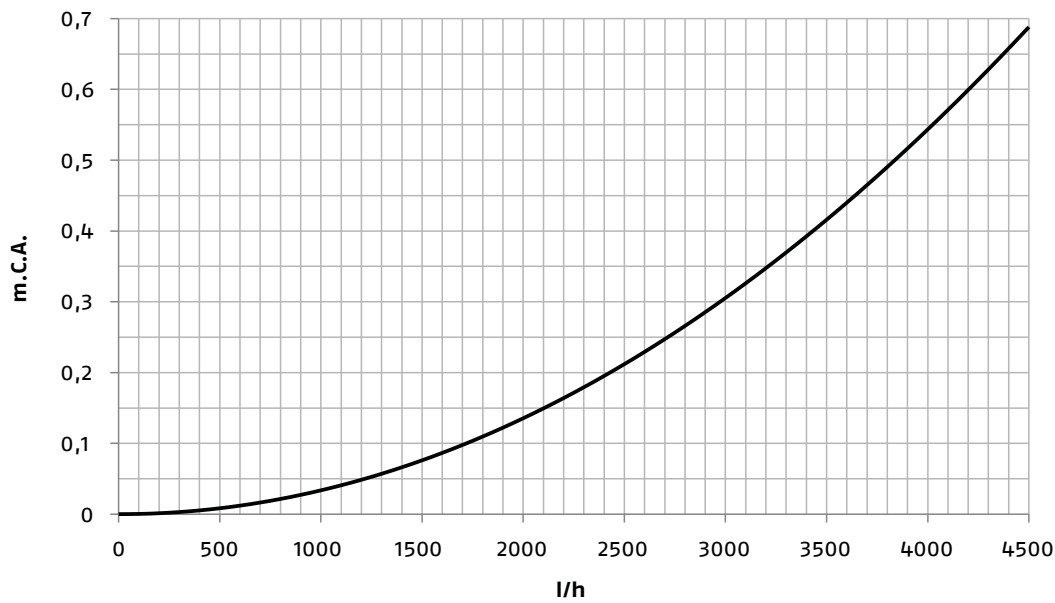
HEAD LOSS
