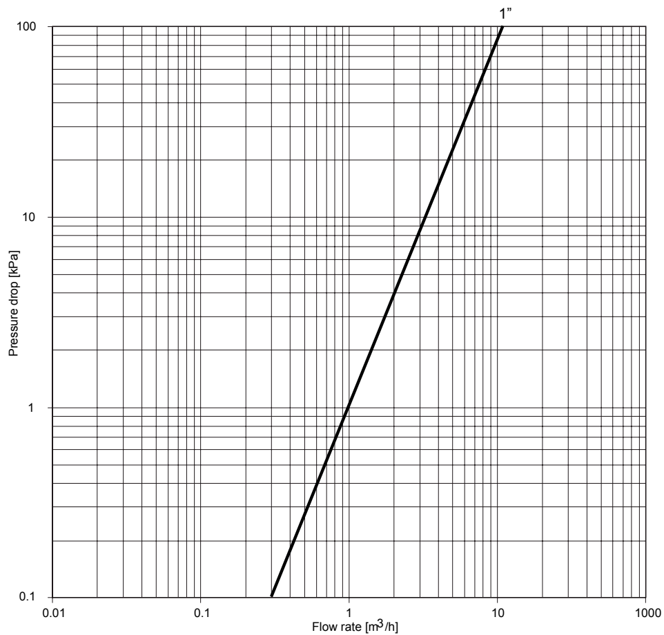
HEAD LOSS
