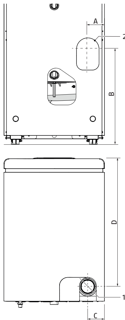
TAU UNIT 50 - 70 - 100 - 115
