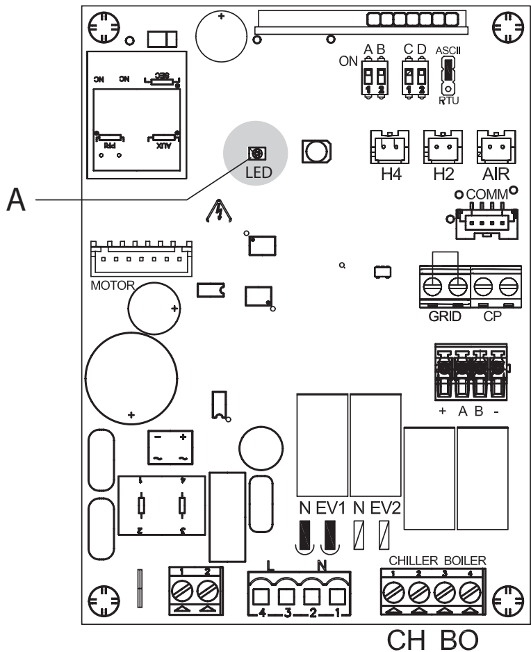
LED SIGNALS (ref. A)
