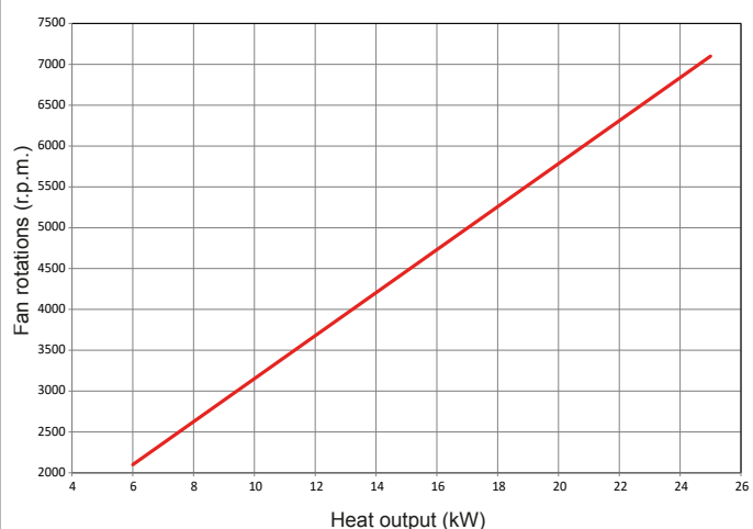
THERMAL OUTPUT CURVE - NO. OF FAN ROTATIONS (MTN)
