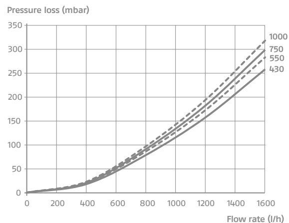
RIELLO 7200 KOMBISOLAR2S LOWER COIL
