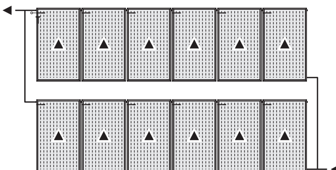
Horizontal configuration
