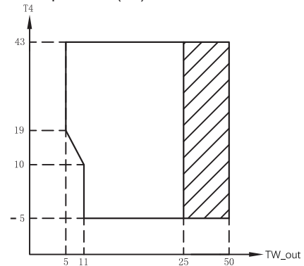
Operation range by heat pump with possible limitation and protection.
