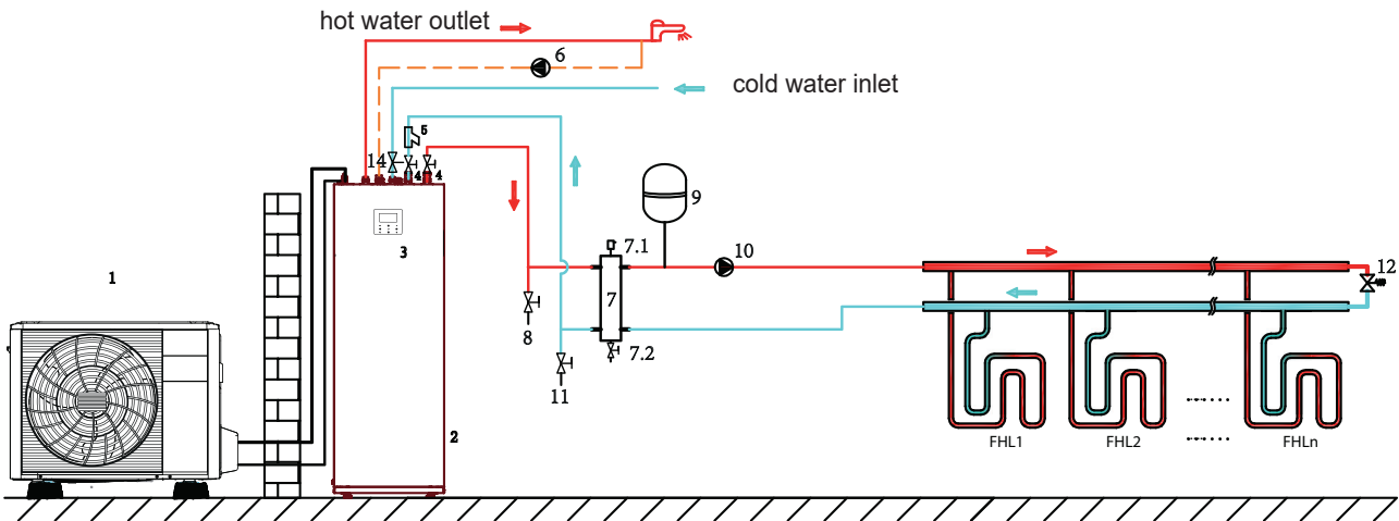
One zone for floor heating loops
