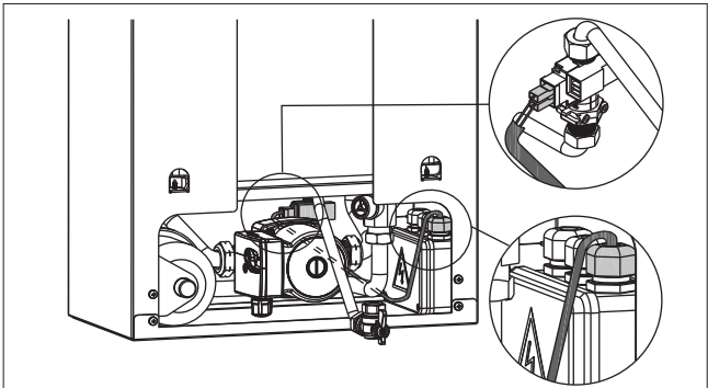
FACTORY CONFIGURATION – FLOW SWITCH CONNECTION
