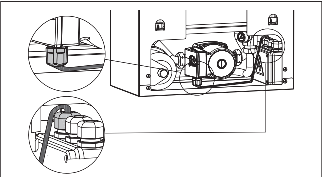
FACTORY CONFIGURATION – CIRCULATOR CONNECTION
