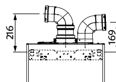
Ø80-80 fixed
