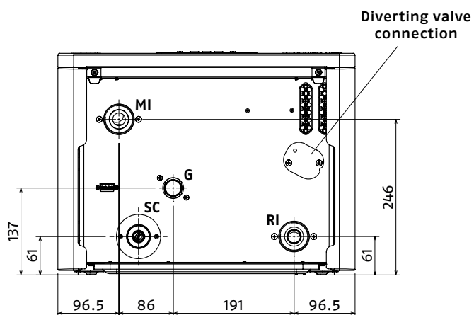
CONDEXA HPR 35 - 45
