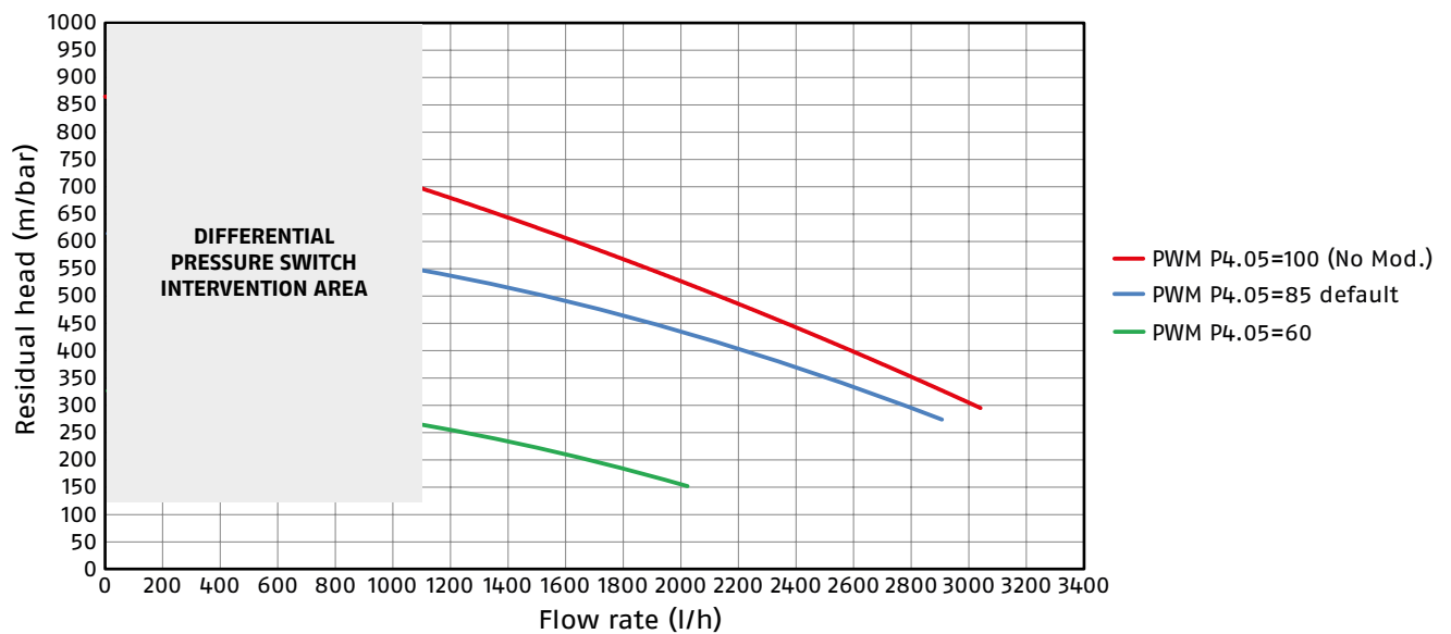
CONDEXA HPR 55 - 70
