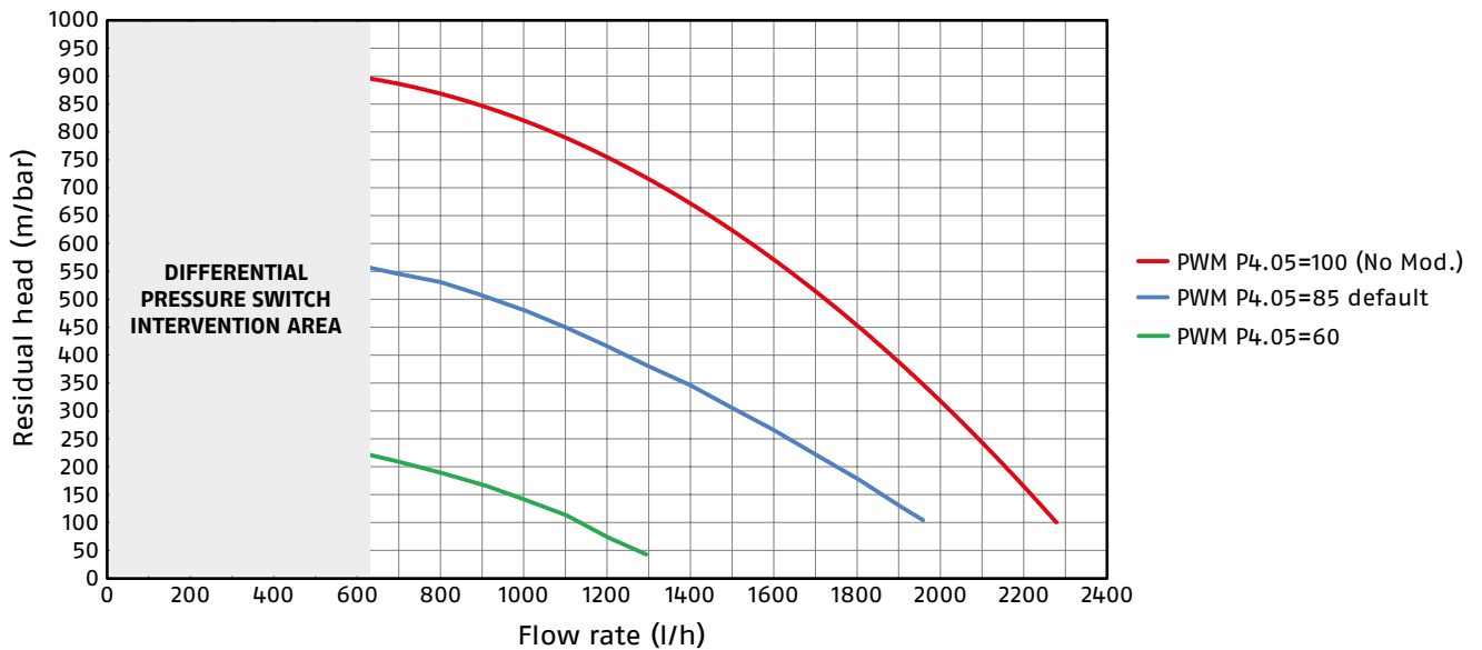
CONDEXA HPR 35 - 45
