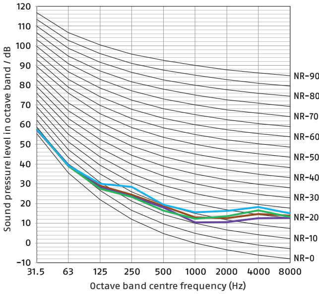
Cooling A35W18
