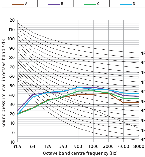
Heating A7W35
