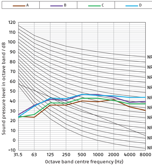
Cooling A35W18
