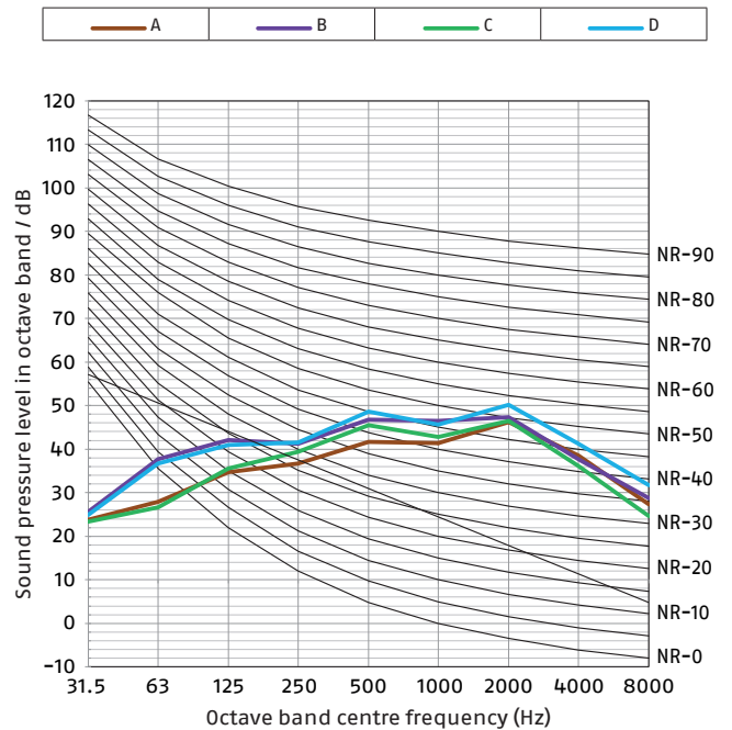
Cooling A35W7
