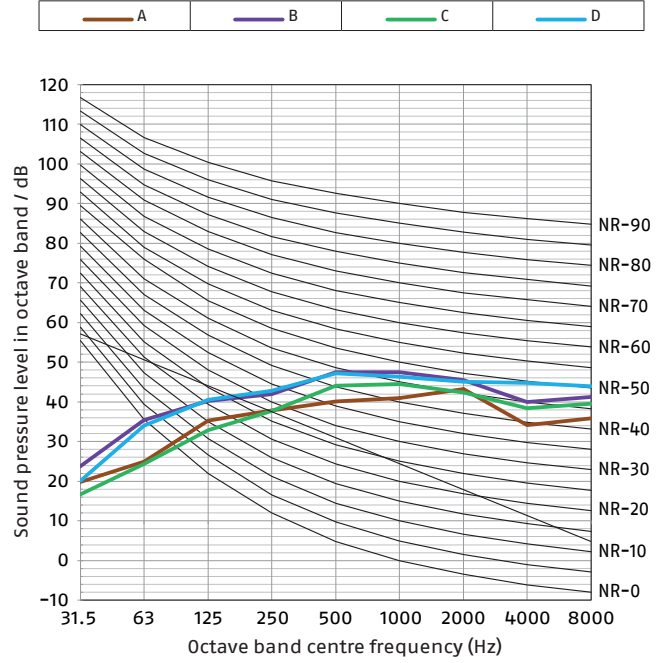
Heating A7W45
