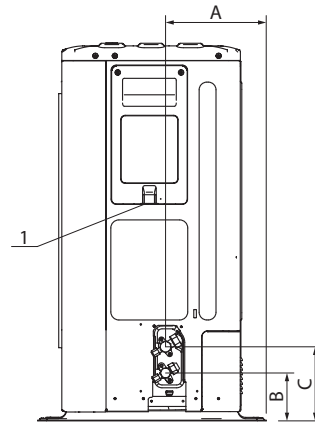
HP EXTERNAL UNIT 008÷016 - 012T÷016T
